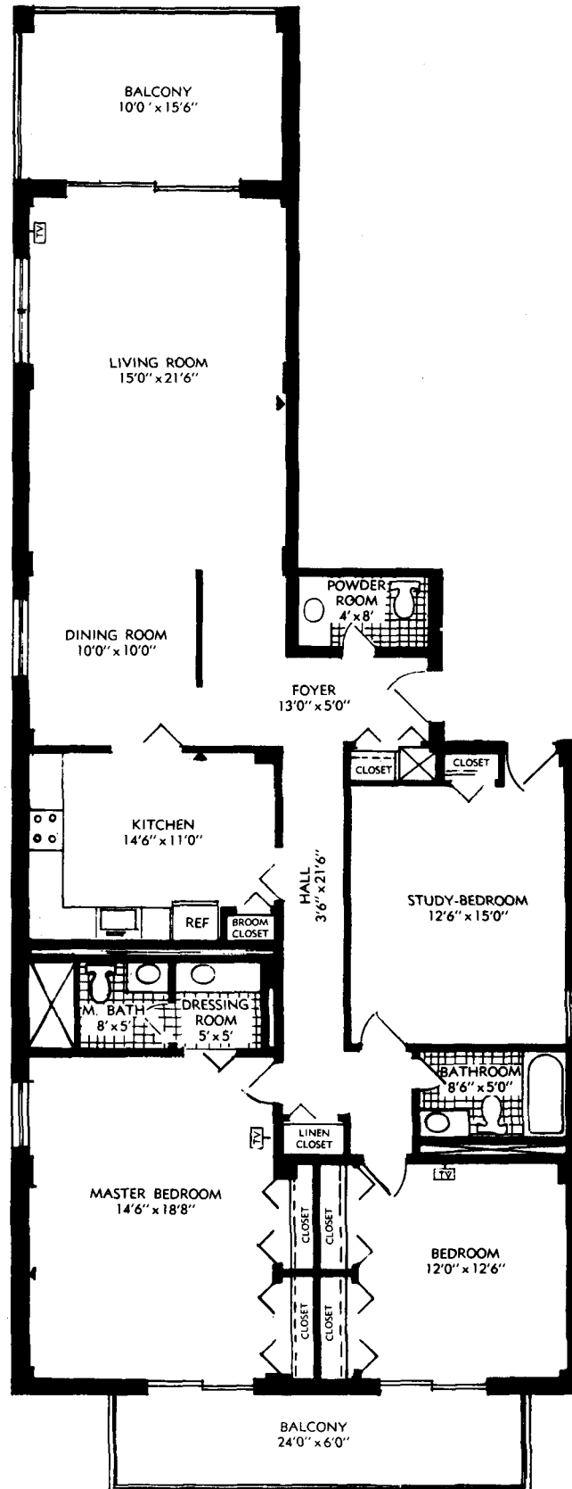
TYPICAL 3 BEDROOM FLOOR PLAN
